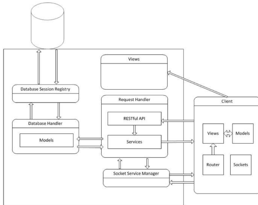
Figure 2 Software architecture
